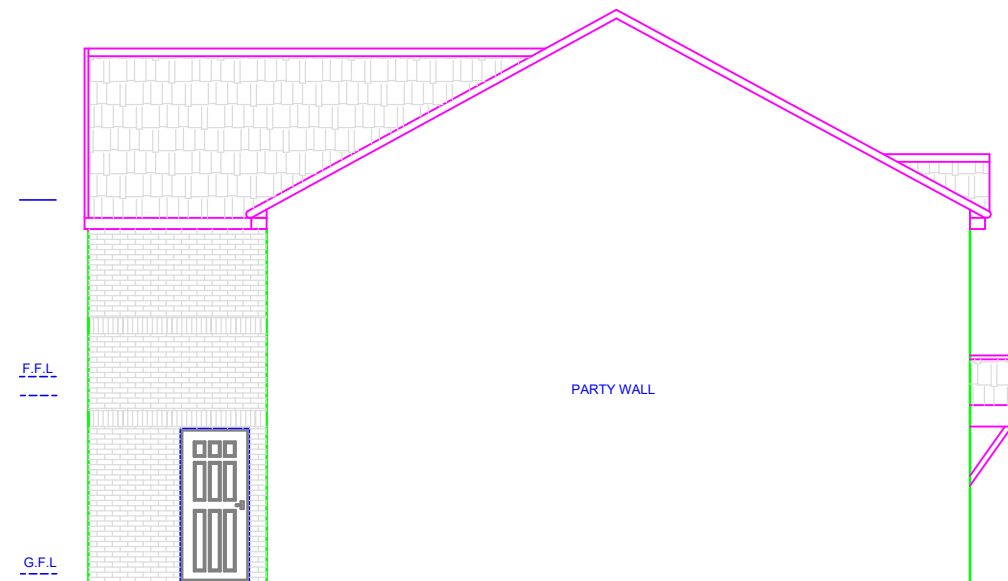
EXISTING SIDE ELEVATION (NORTH EAST)
