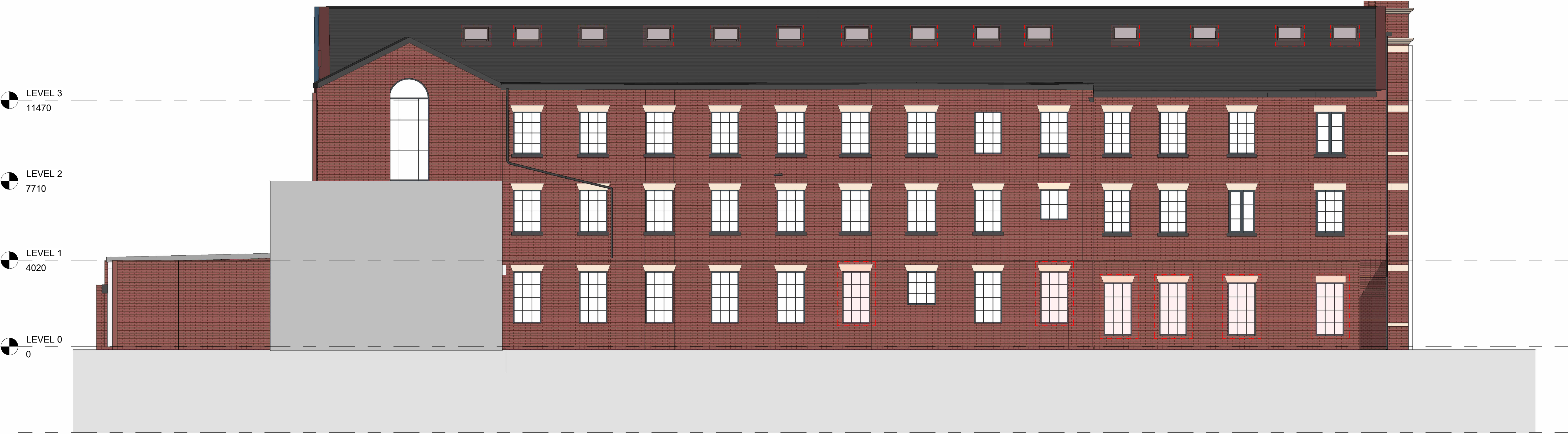
1 Rear - Proposed 1 : 100
