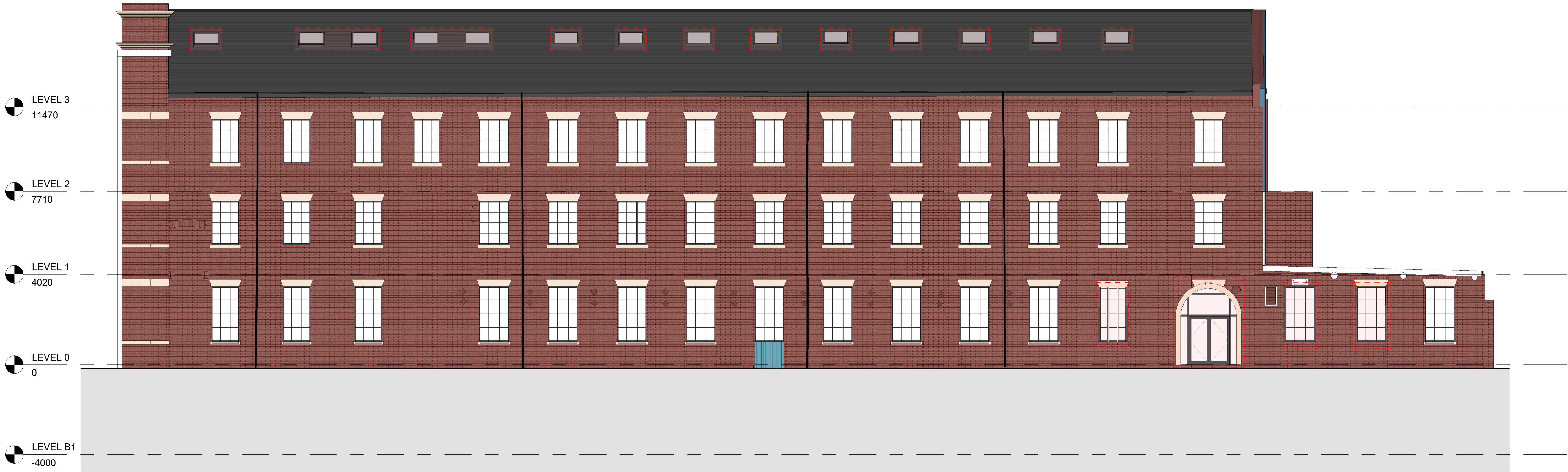
1 Front - Proposed 1 : 100
