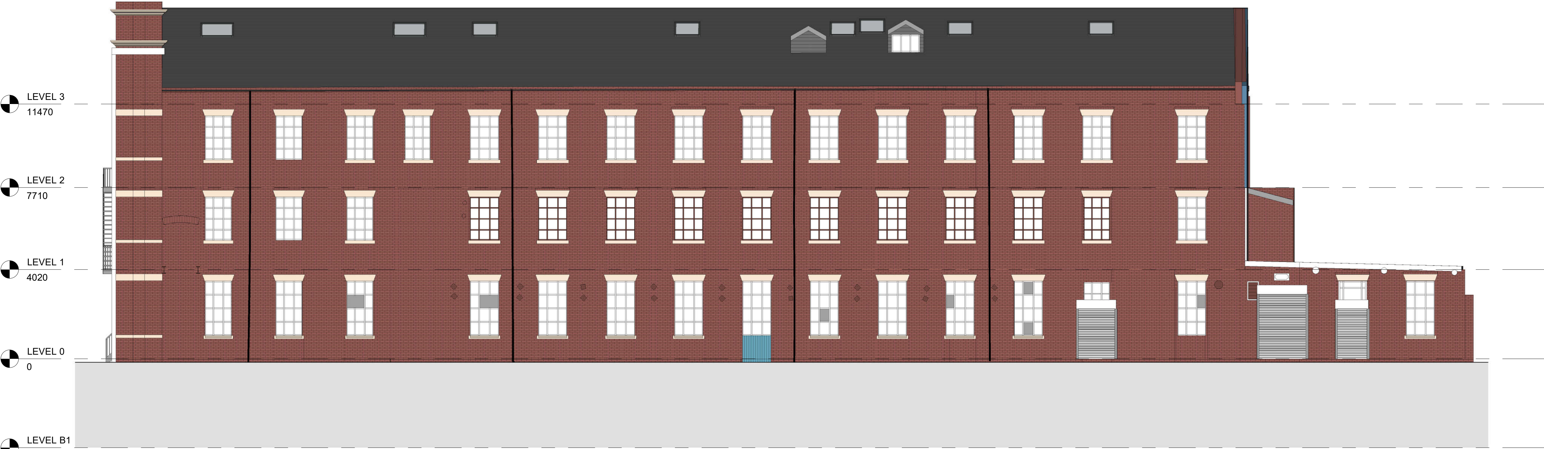
1 Front - Existing 1 : 100
