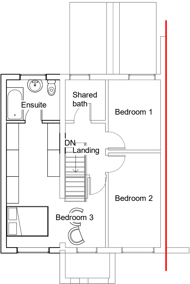
4 First Floor - Proposed 1 : 100
