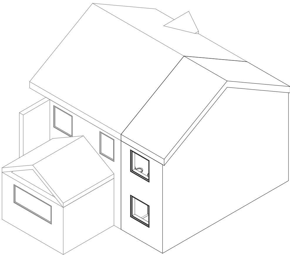
4 Iso- Rear Proposed
