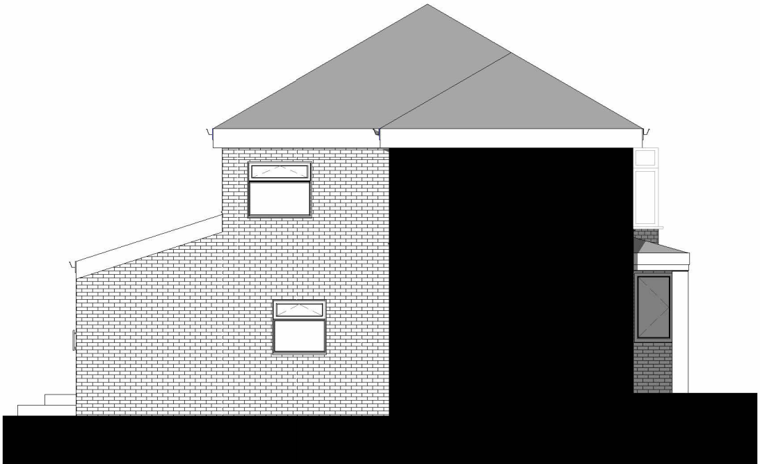
EXISTING SIDE ELEVATION 1:100 @ A3
