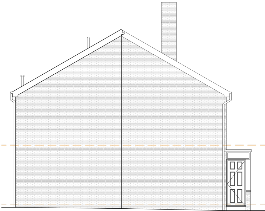
Side Elevation 1:100 @ A3
