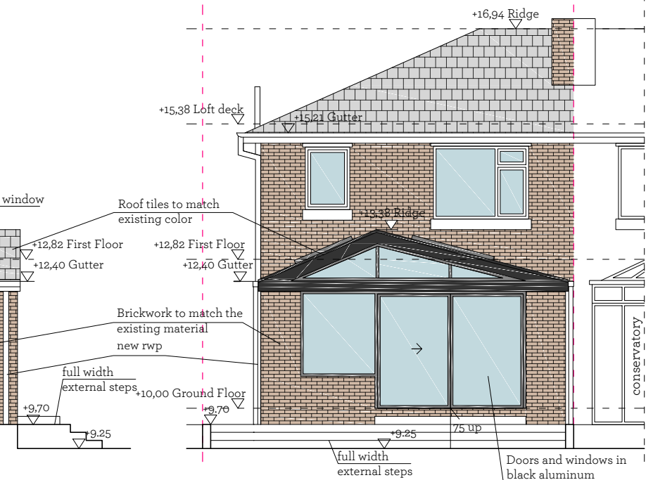
Proposed Western Elevation
