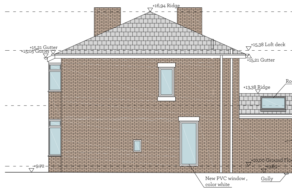
Proposed Northern Elevation
