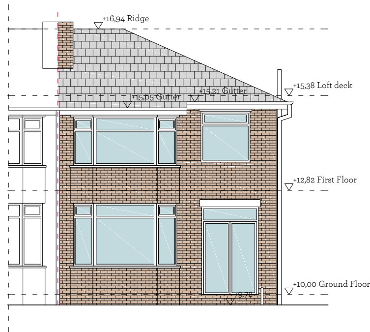
Eastern Elevation (Front)
