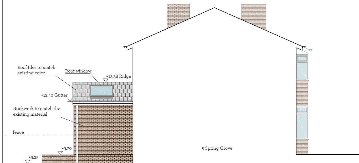
Side elevation, view from 5 Spring Grove.
