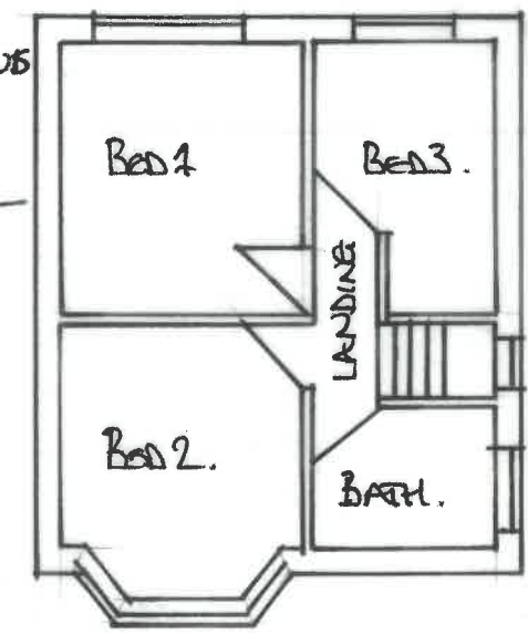
EXISTING FIRST floor 1-100
