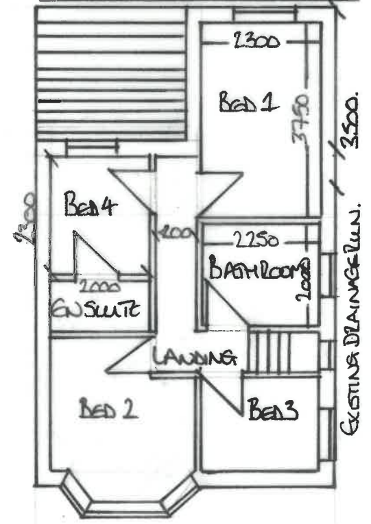
PROPOSED FIRST floor 1-100
