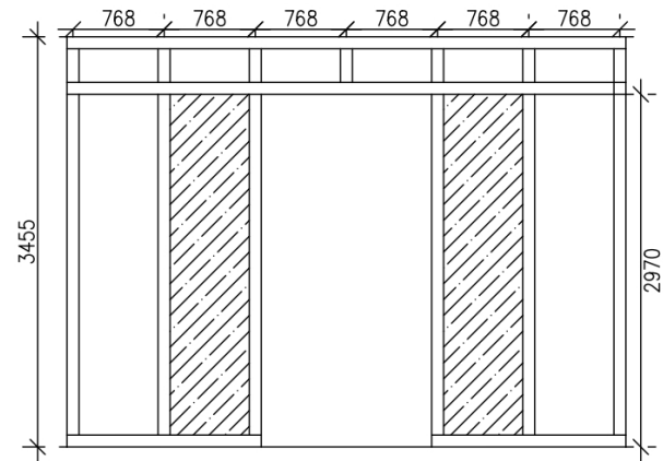
TYPICAL PLASTERBOARD DRYWALL CONSTRUCTION WITH DOOR OPENING
