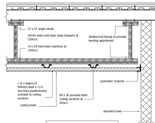
Suspended Ceiling Detail
