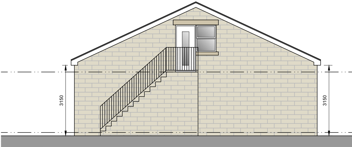
South Facing Rear Elevation
