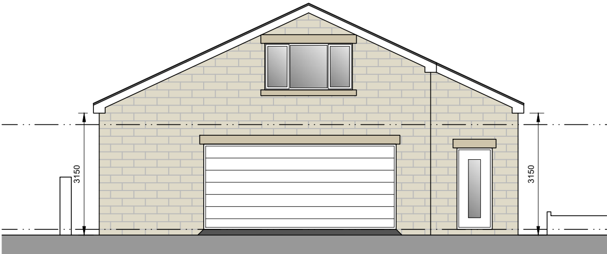
North Facing Front Elevation
