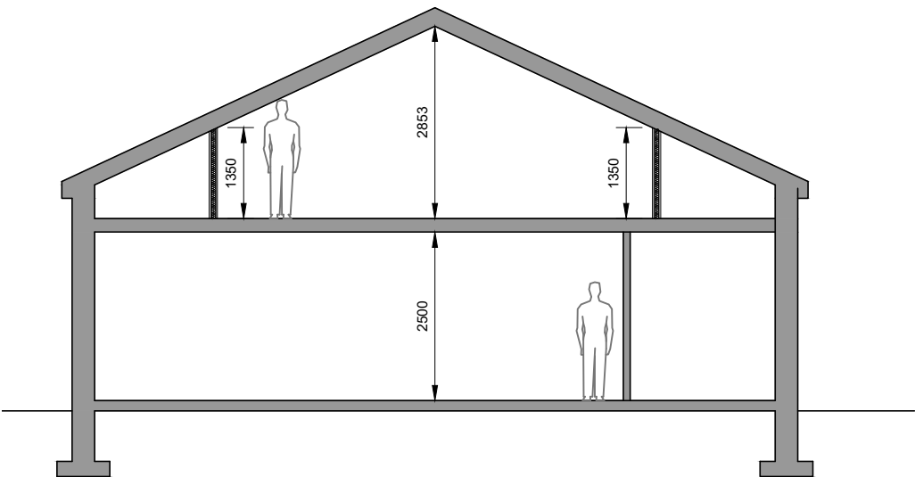
GA Cross Section
