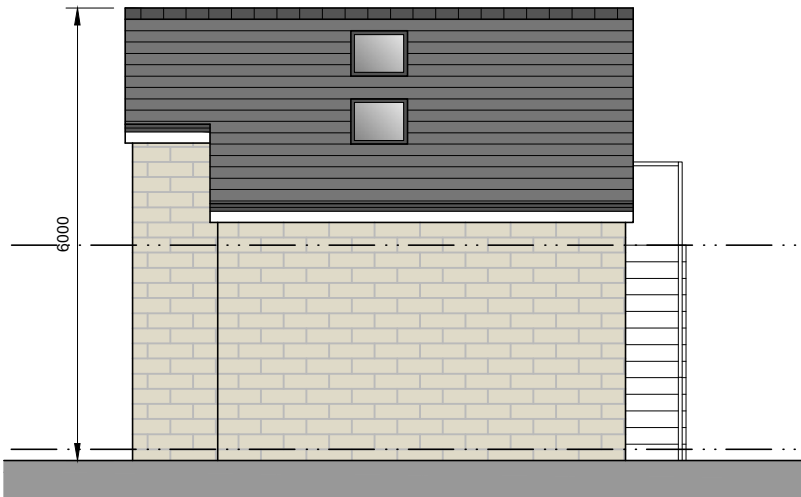
West Facing Side Elevation
