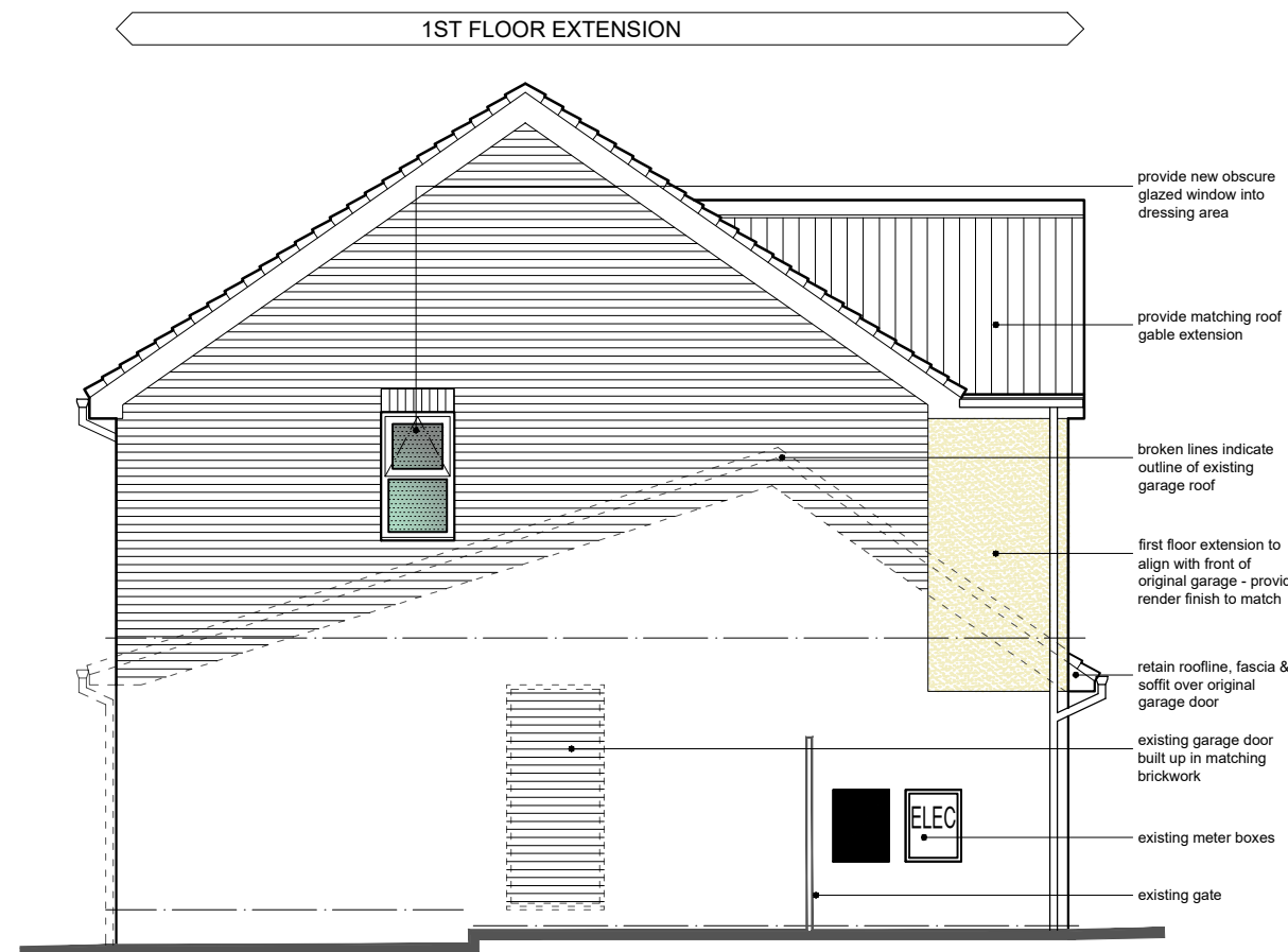
PROPOSED SIDE ELEVATION (facing 3 Stanford hall Crescent)
