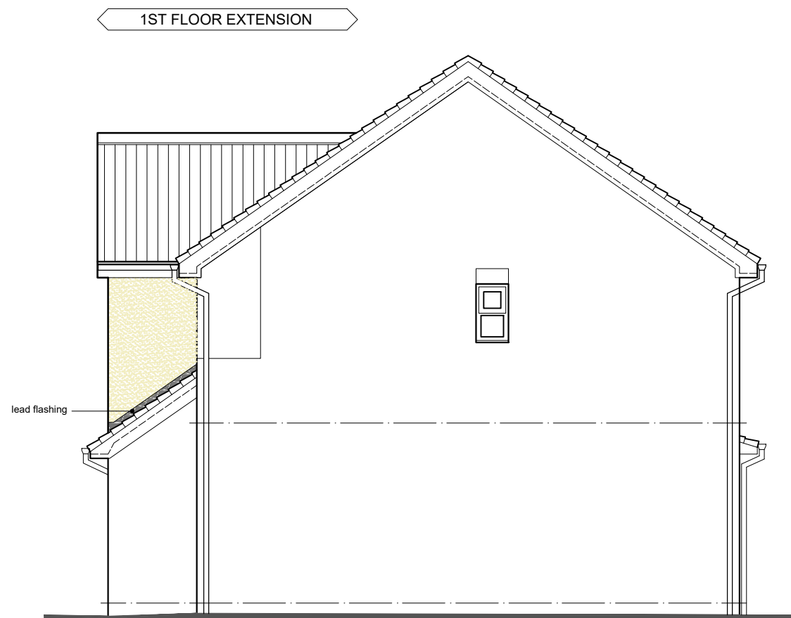
PROPOSED SIDE ELEVATION (facing 5 Stanford hall Crescent)
