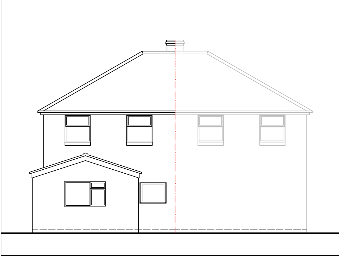
ELEVATION - REAR
