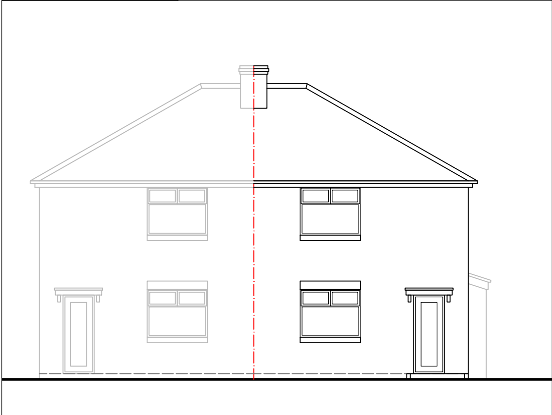
ELEVATION - FRONT
