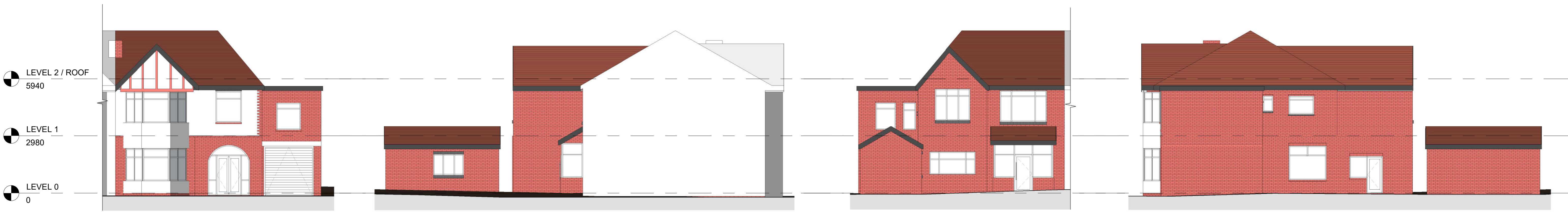
3 Front - Existing 1 : 100
