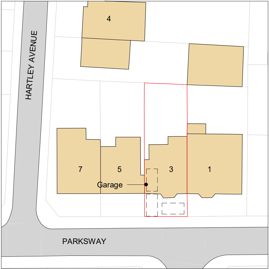
2. Site - Proposed Parking 1 : 500
