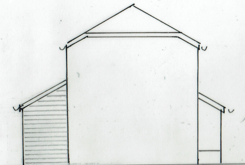
SIDE
