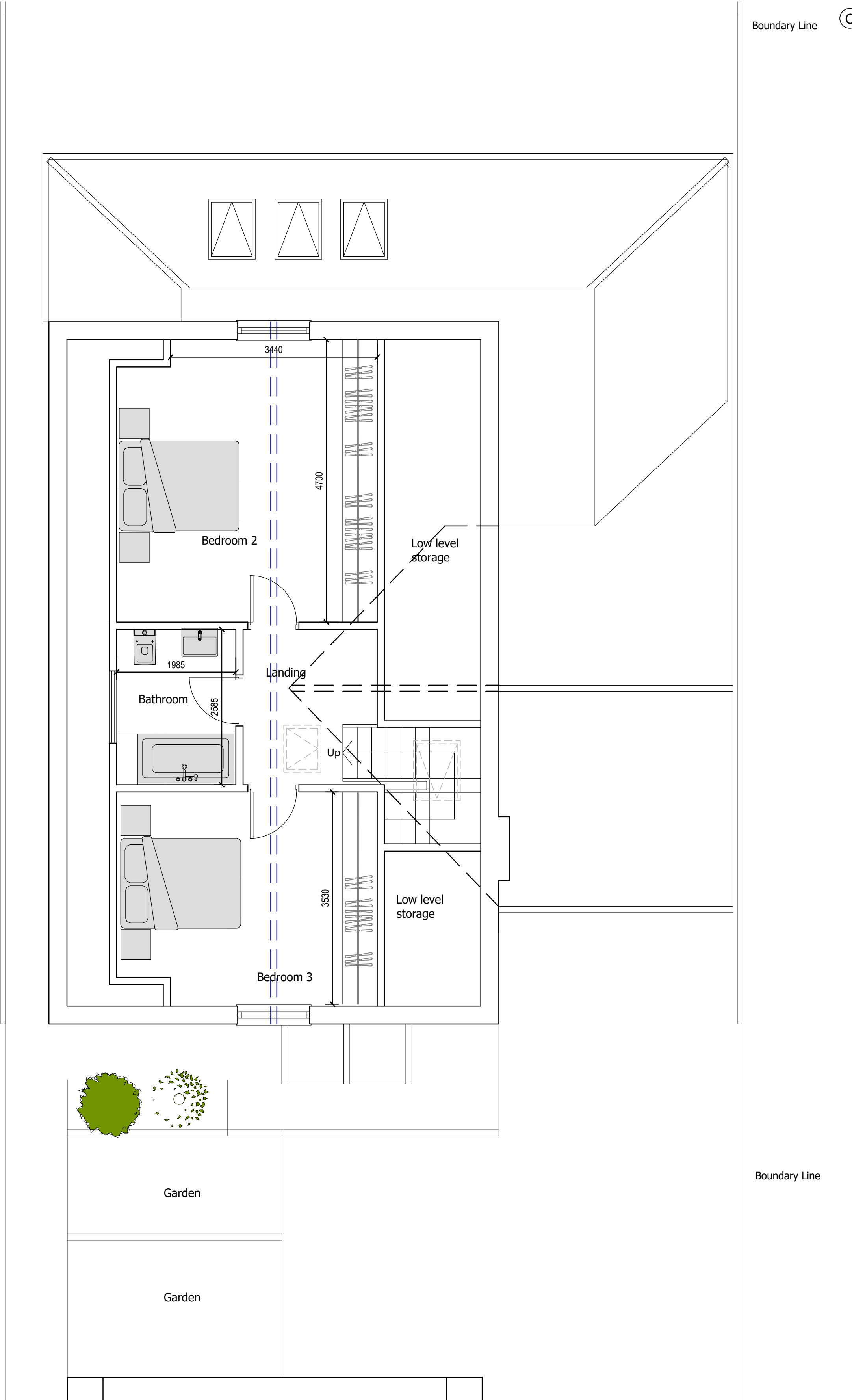
First Floor
