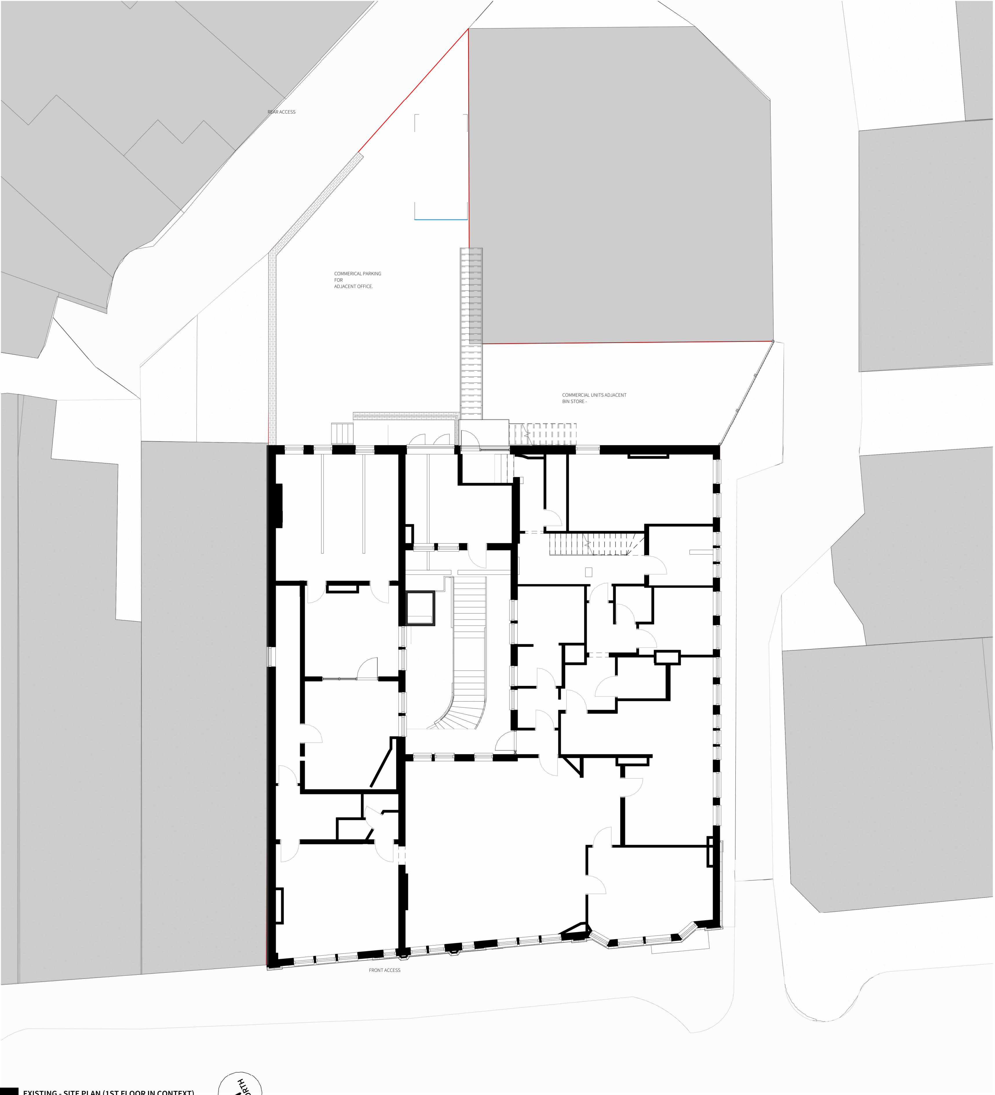
1 EXISTING - SITE PLAN (1ST FLOOR IN CONTEXT) 1:100
