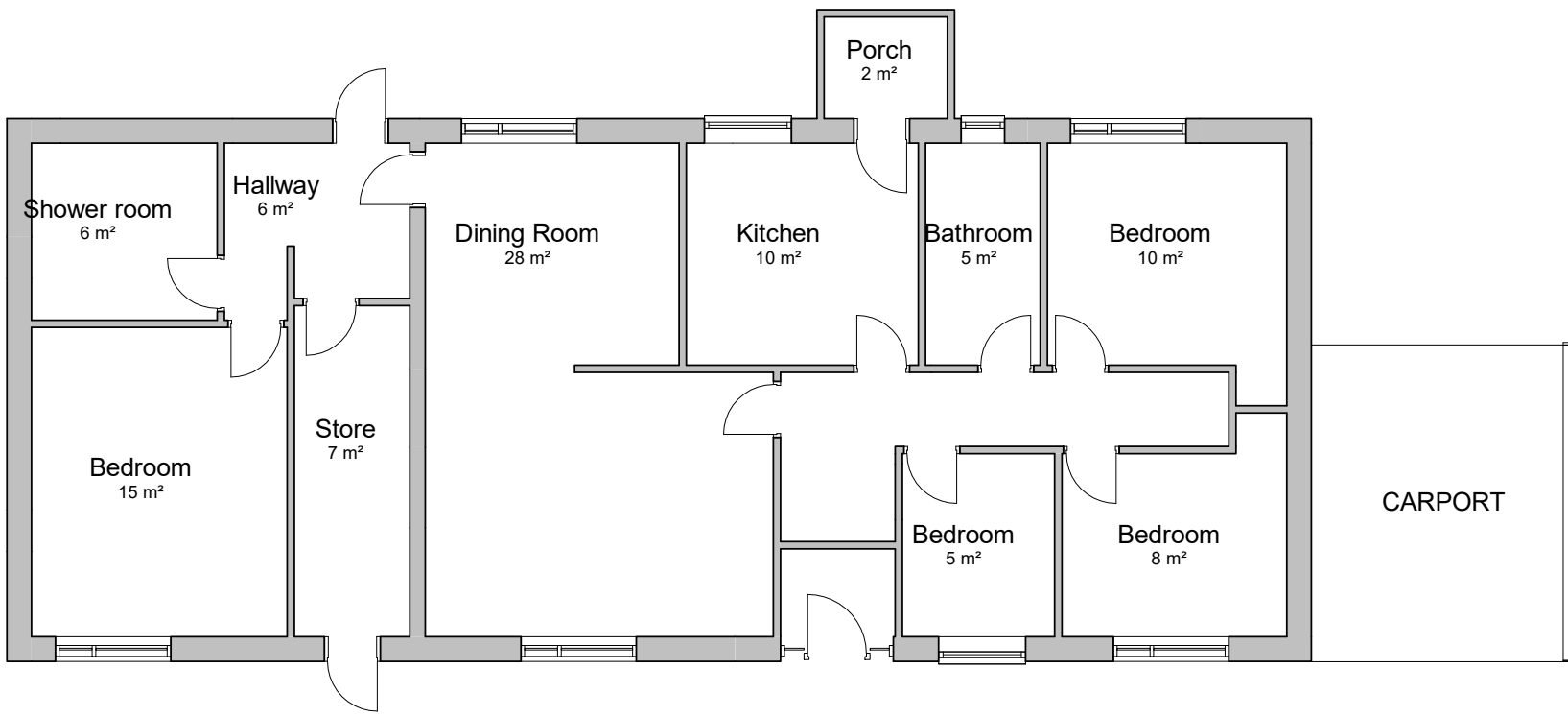
② Level 0 GA Existing 1 : 100
