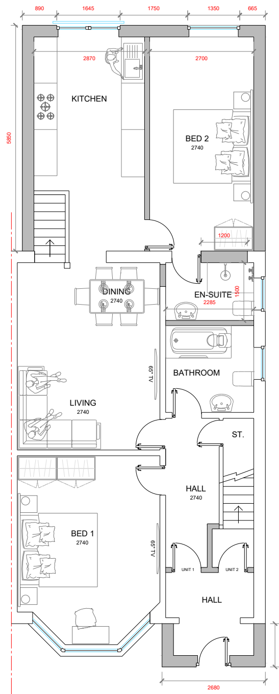
GROUND FLOOR
