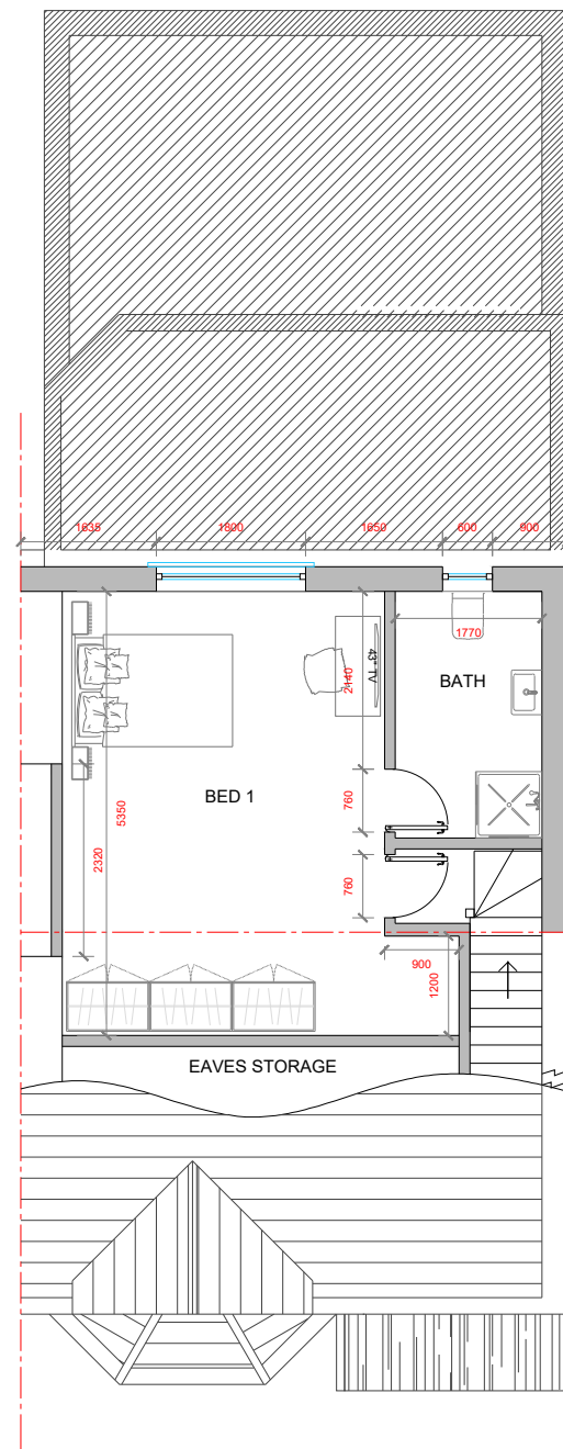
ROOF SPACE
