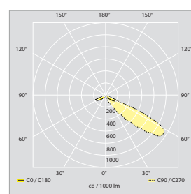
Asymmetrical shield
