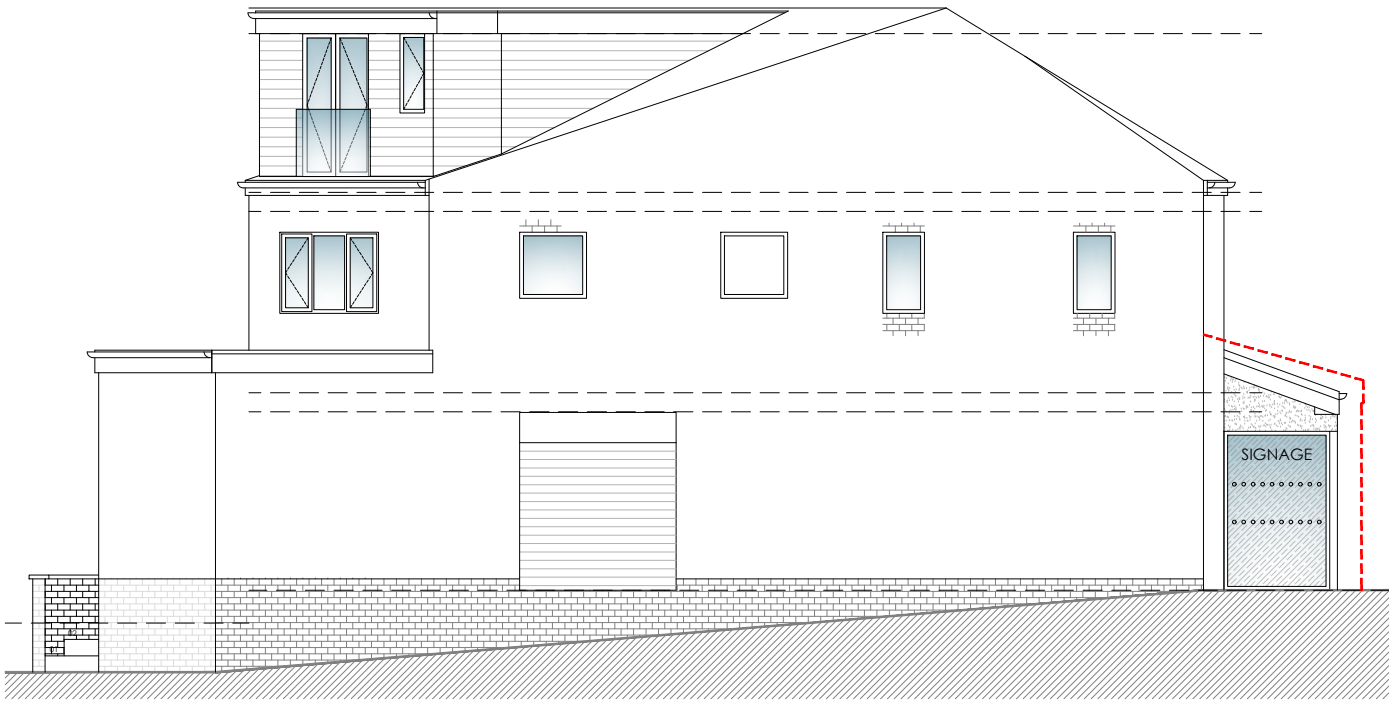
PROPOSED GABLE ELEVATION 1:100
