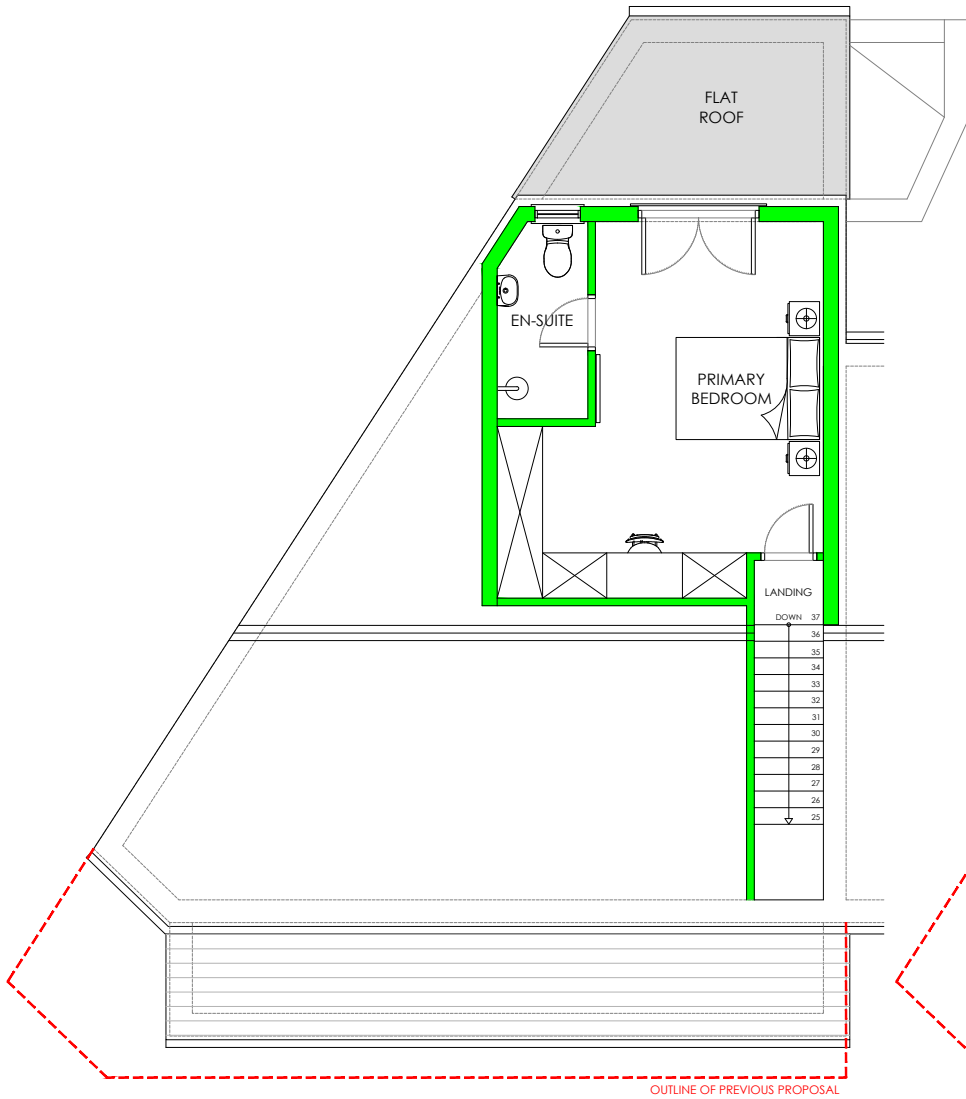
PROPOSED SECOND FLOOR PLAN 1:100
