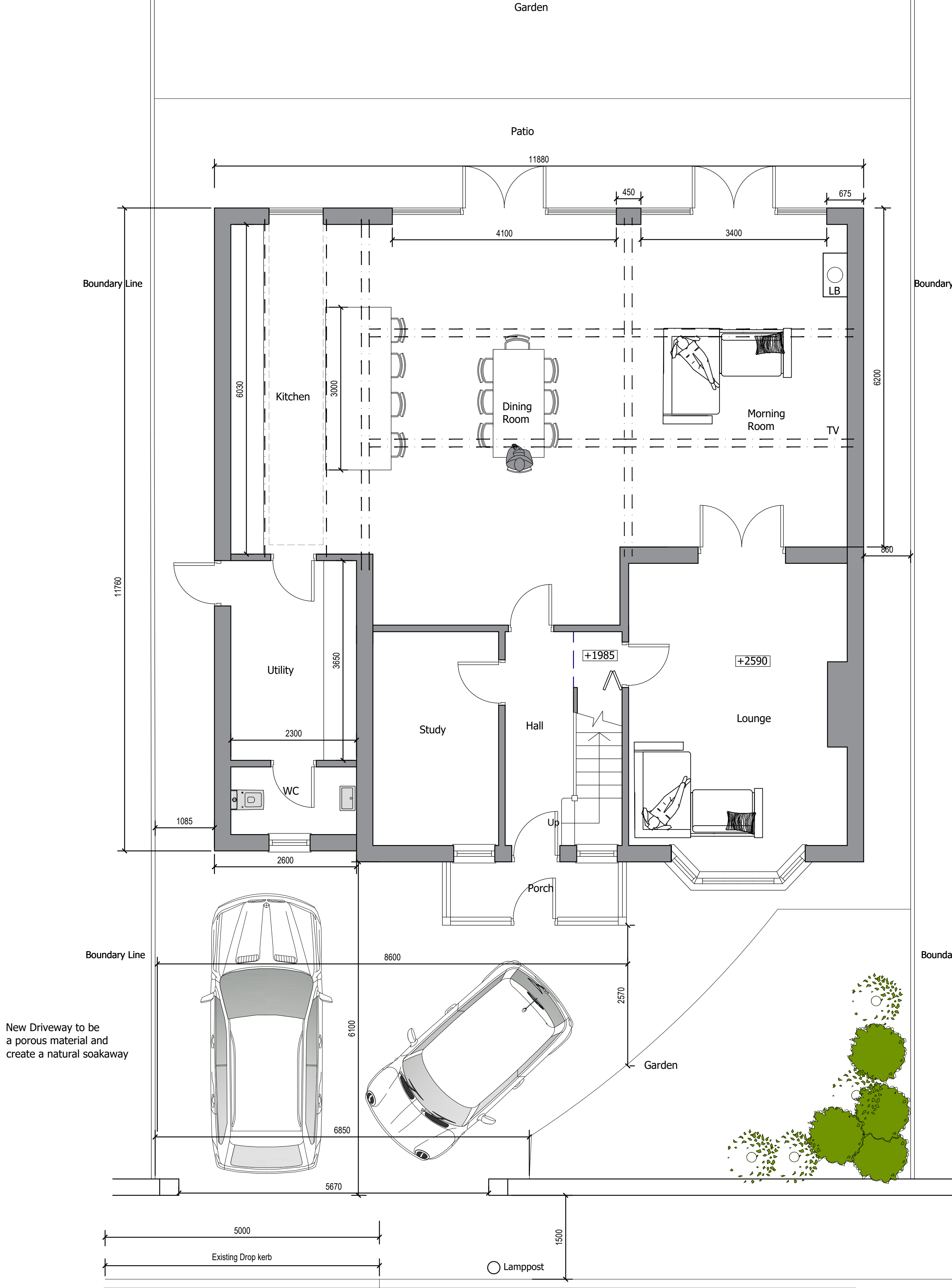
Ground Floor
