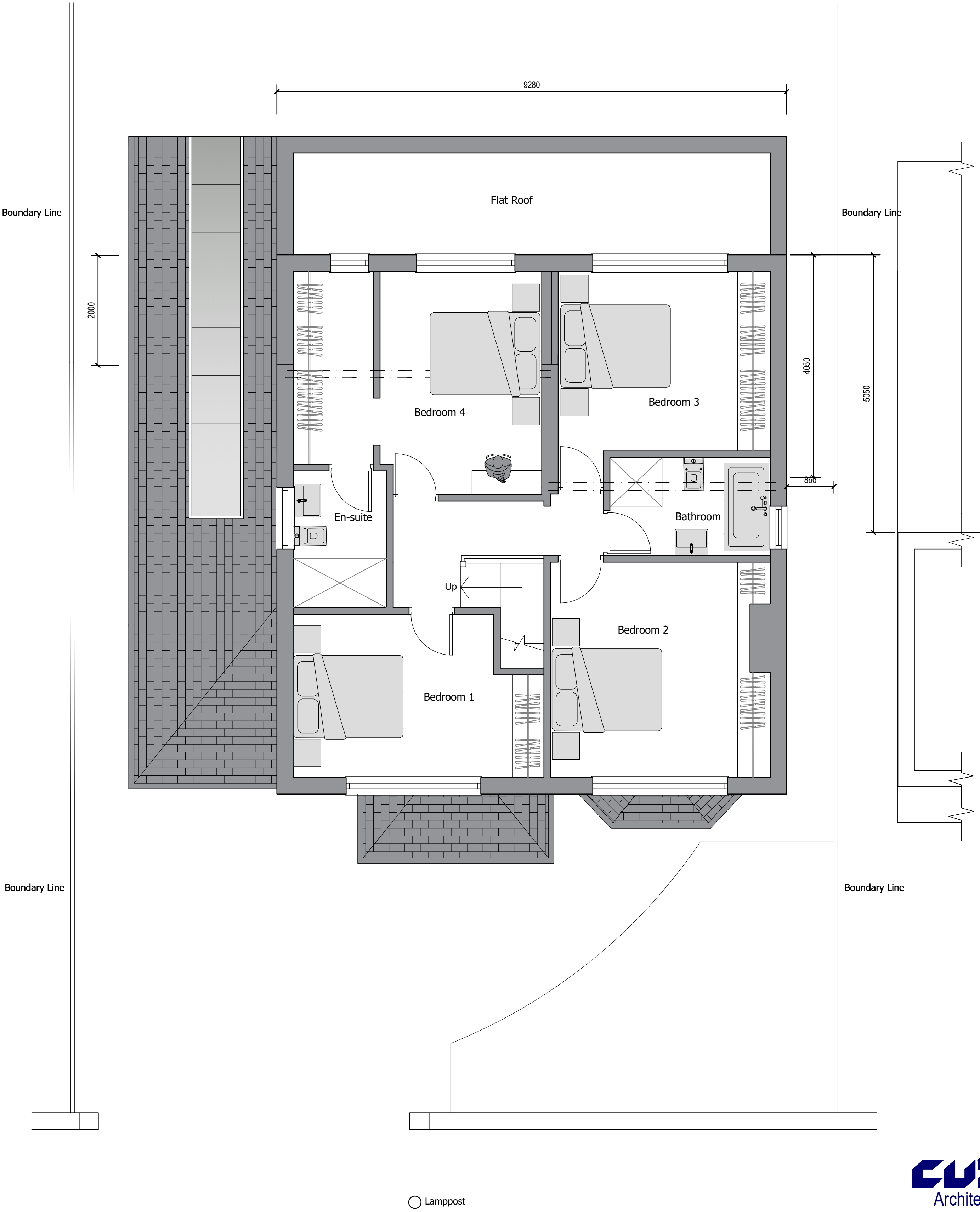
First Floor
