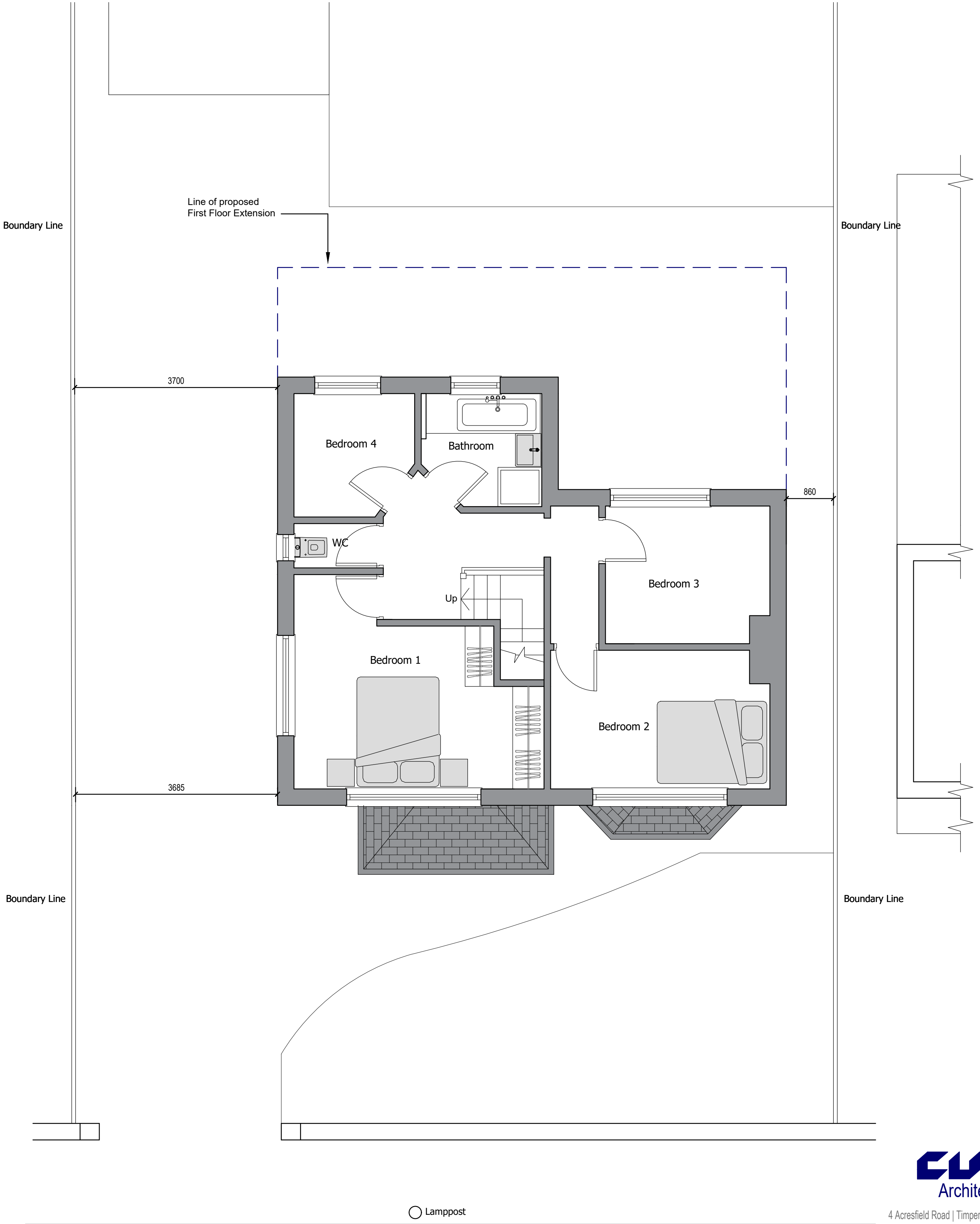
First Floor
