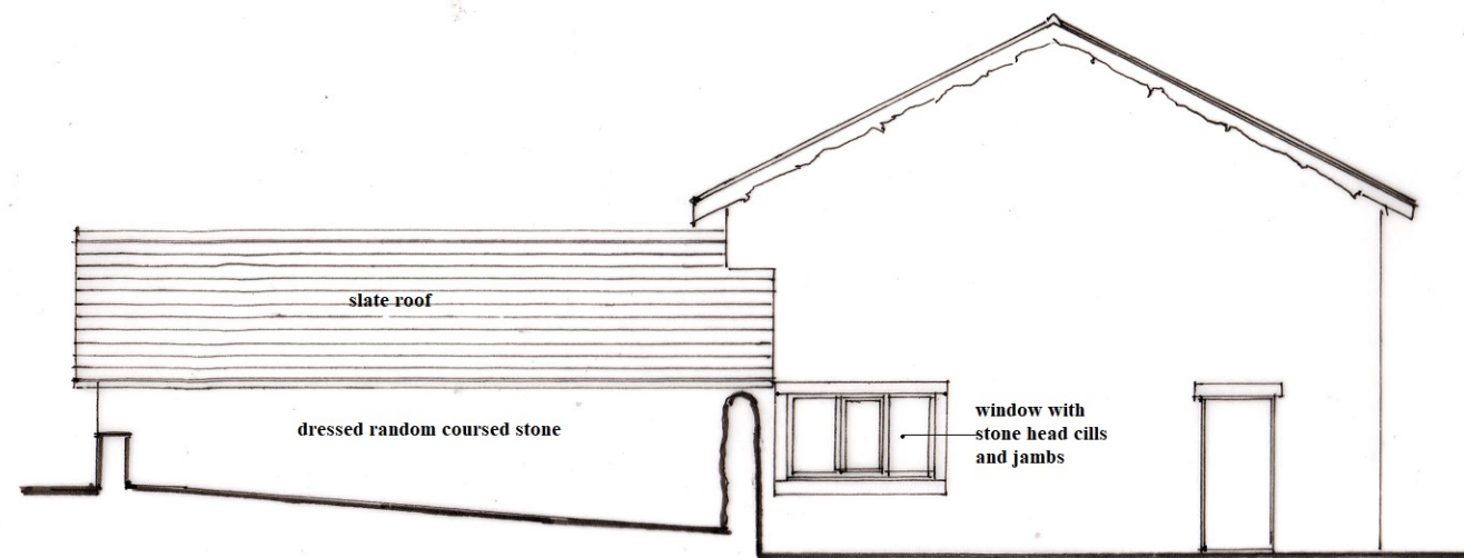
West Elevation
