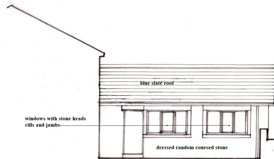
East Elevation
