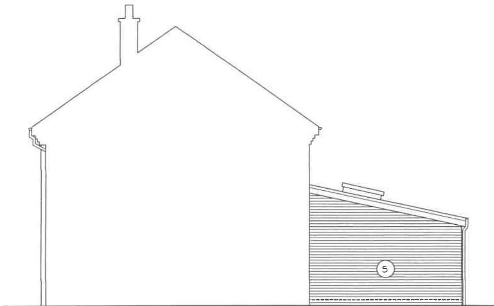
PROPOSED NORTH EAST ELEVATION/SECTION [VIEWED FROM NO. 110] 1:100
