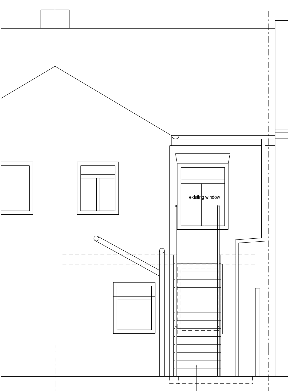
PROPOSED NORTH (REAR ) ELEVATION
