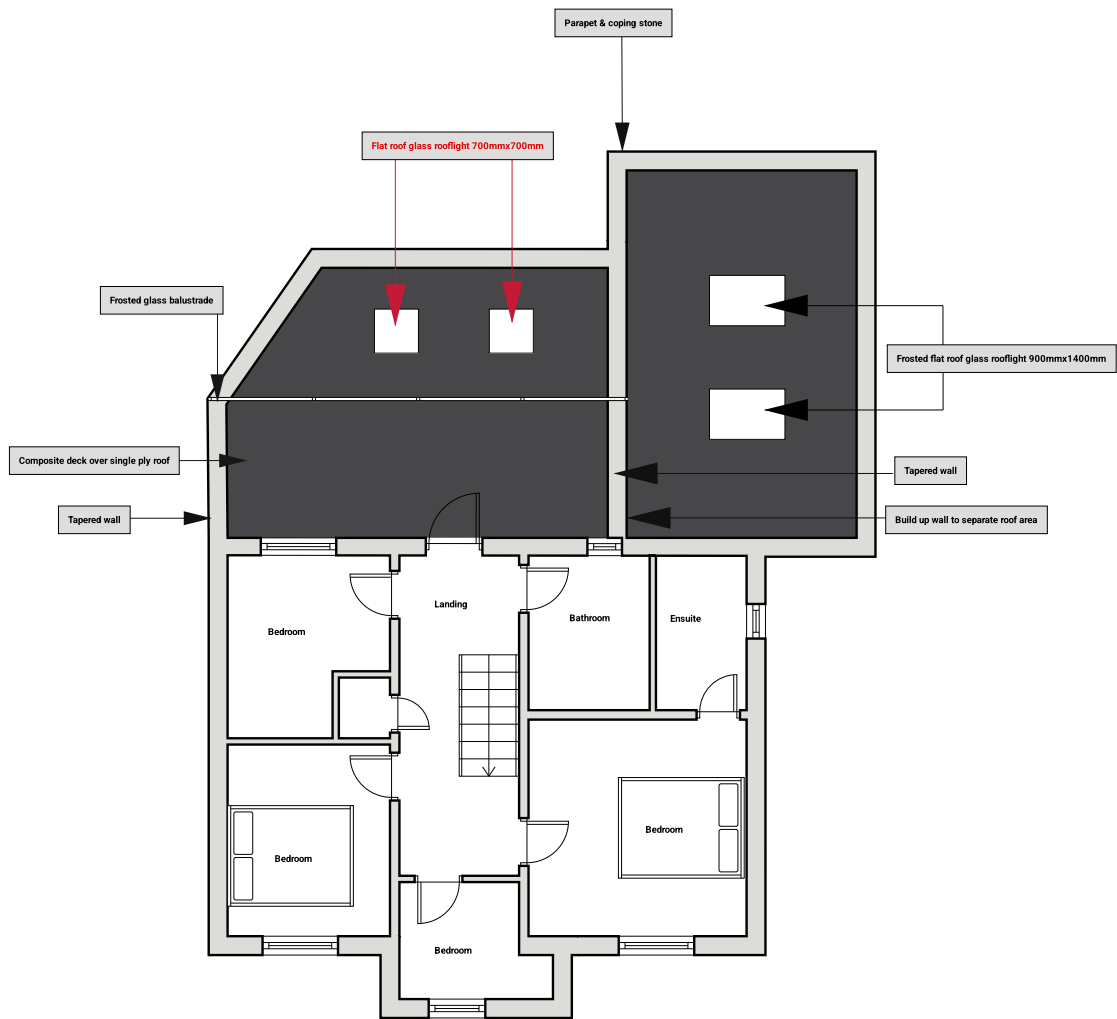
Proposed First Floor Scale 1:50
