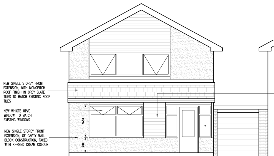
PROPOSED FRONT ELEVATION 1:100 @ A3
