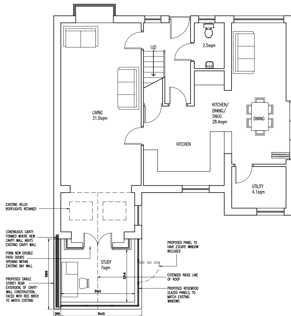
PROPOSED GROUND FLOOR PLAN 1:100 @ A3
