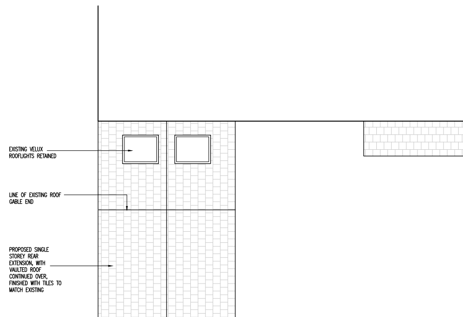
PROPOSED FIRST FLOOR ROOF PLAN 1:100 @ A3
