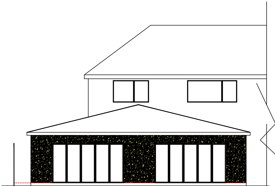
Rear Elevation
