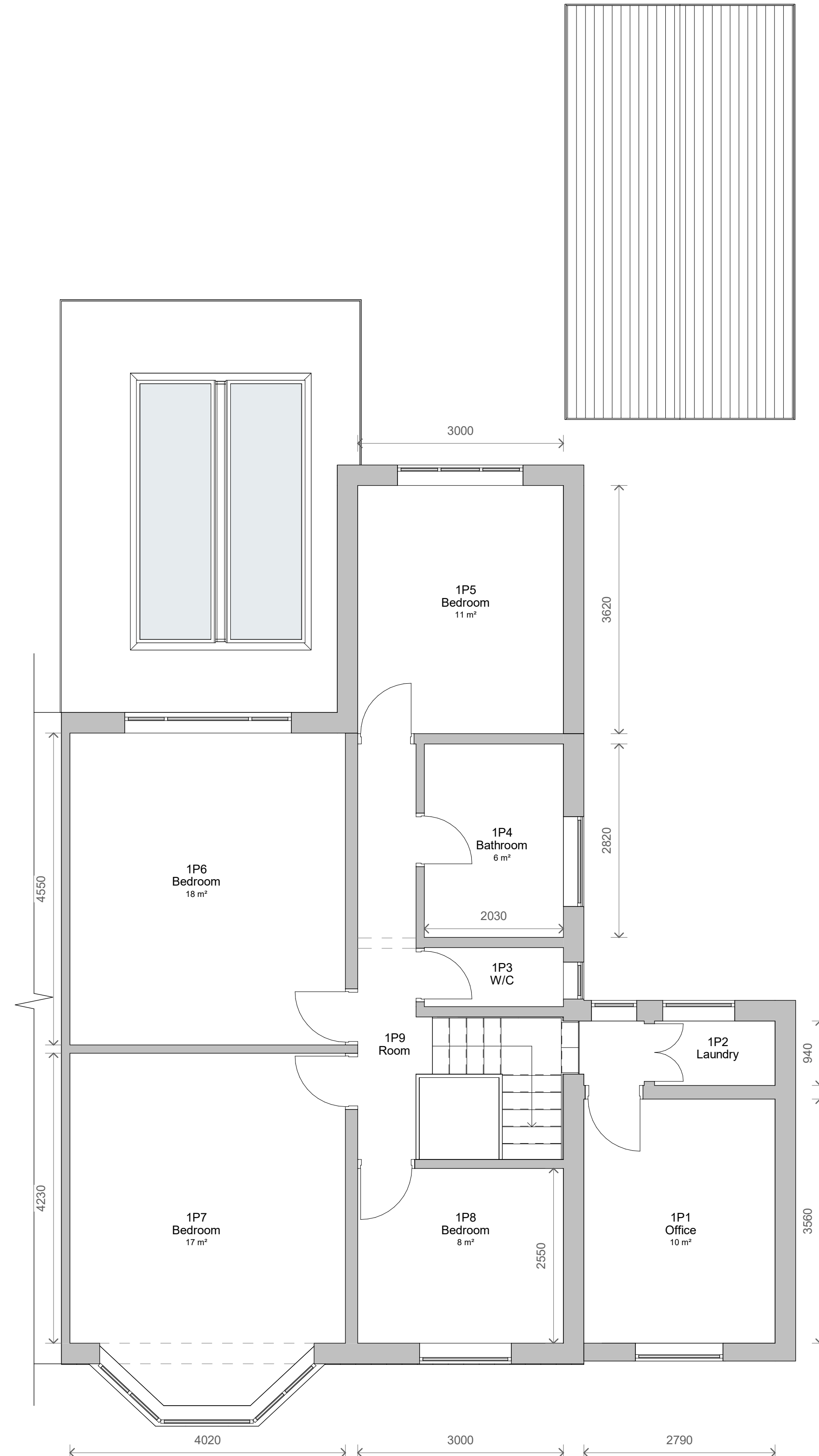
2 Level 1 - Proposed 1 : 50
