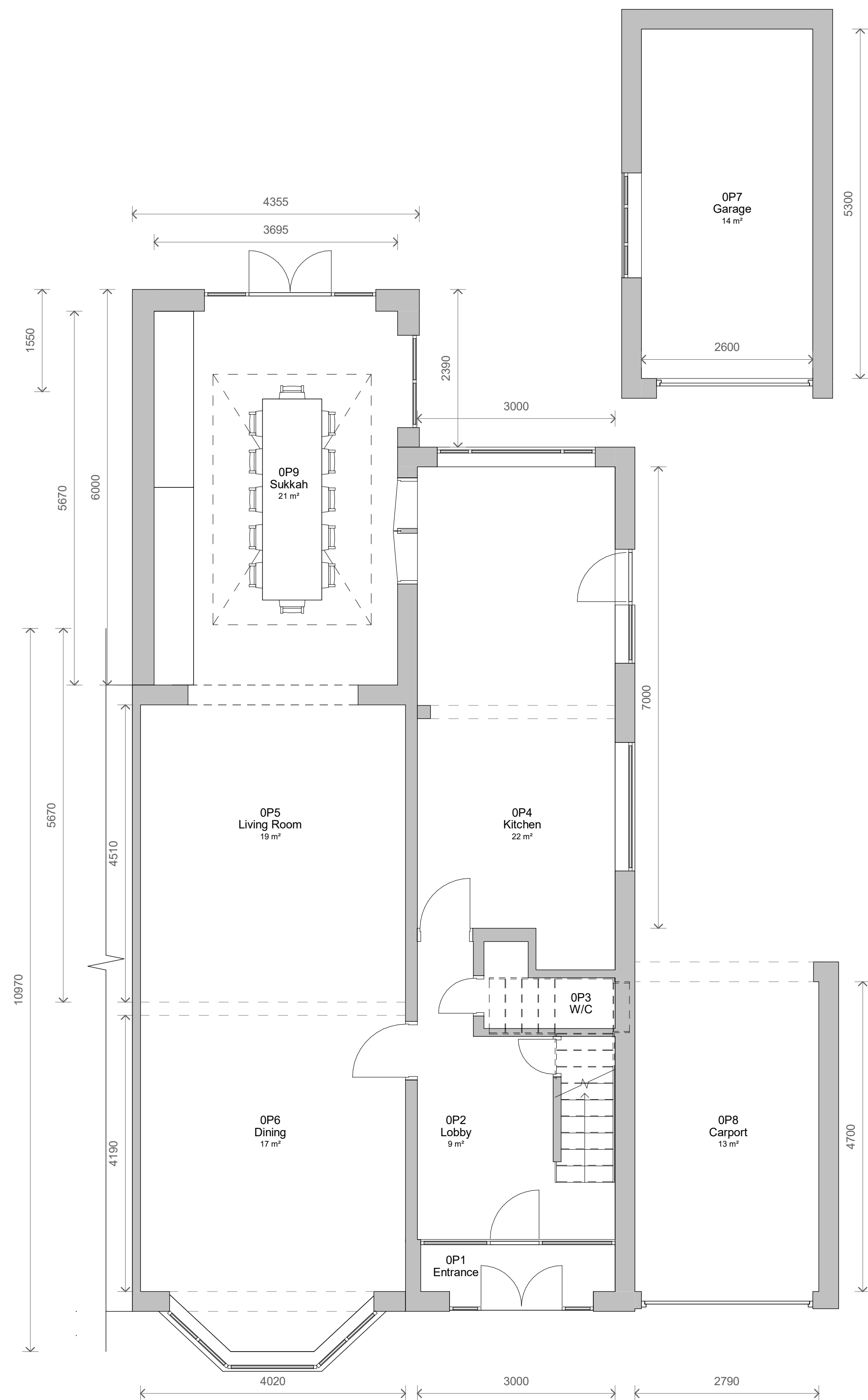
1 Level 0 - Proposed 1 : 50
