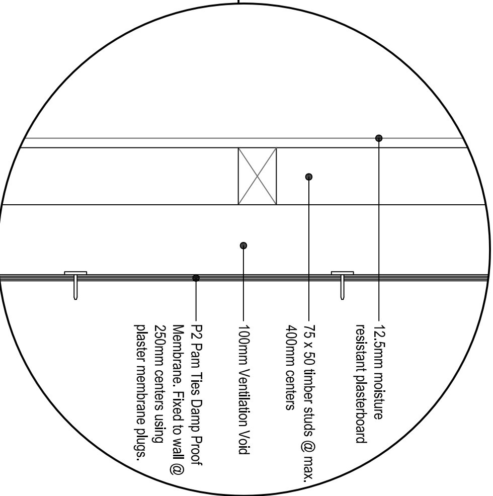
DETAIL 1:5
