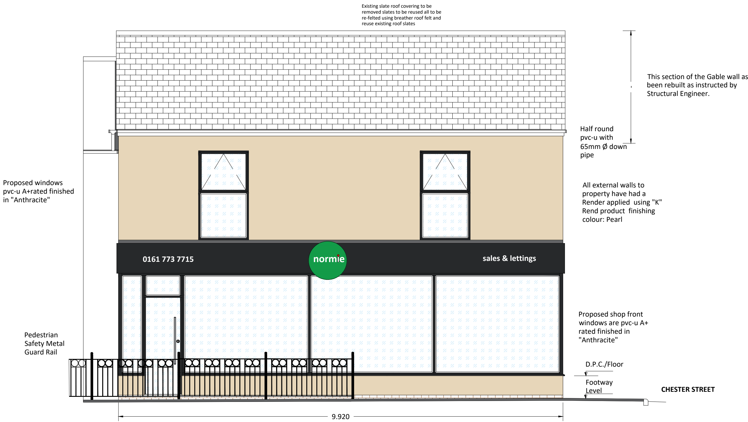
Proposed Front Street View
