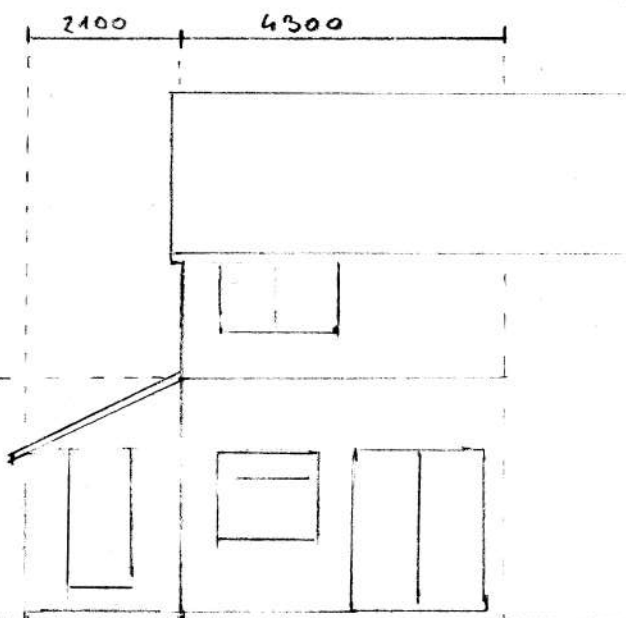
PROPOSED REAR
