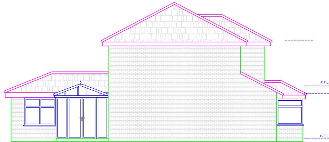
Existing Side Elevation (North West)
