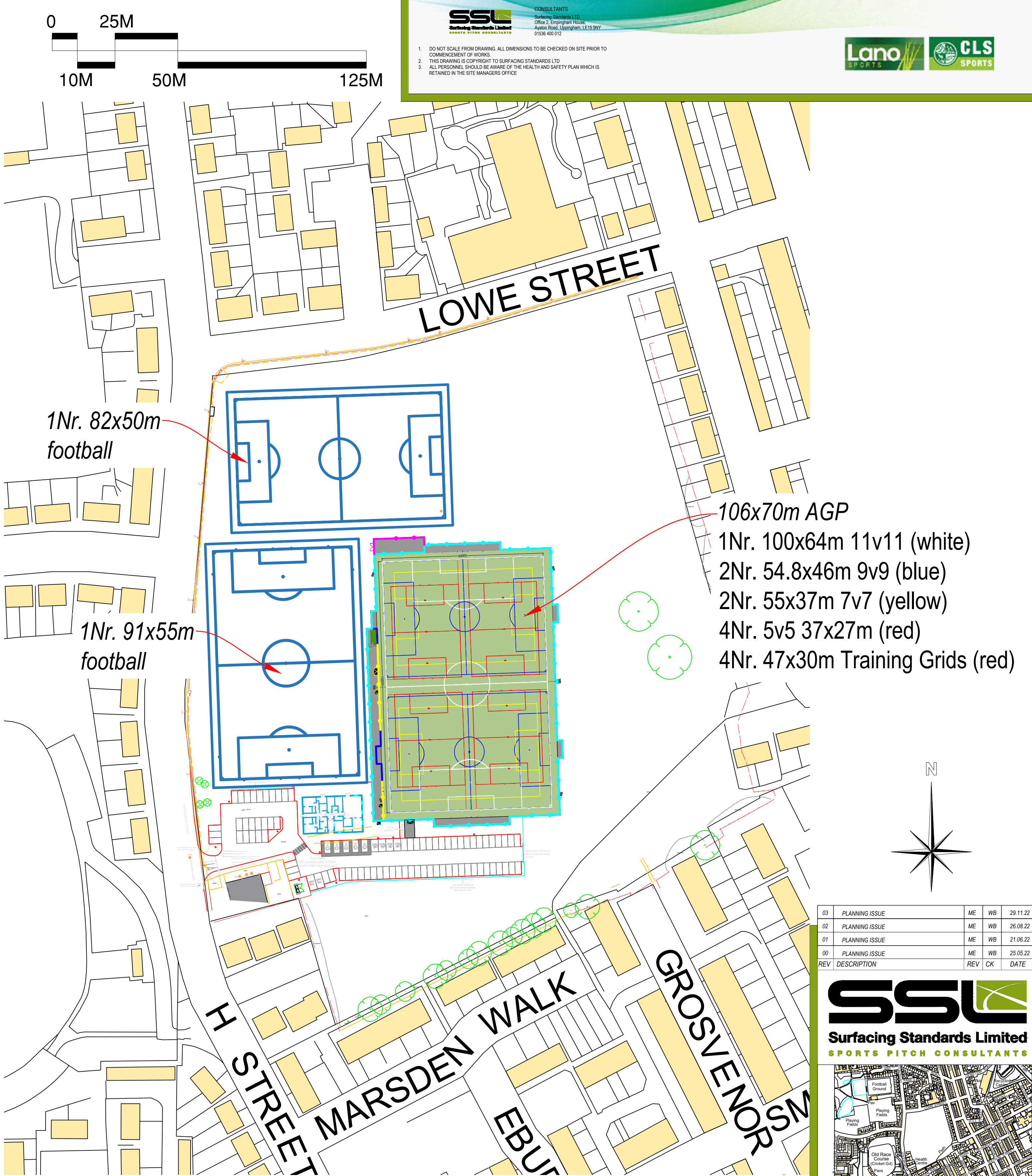
Proposed Playing Field Layout
