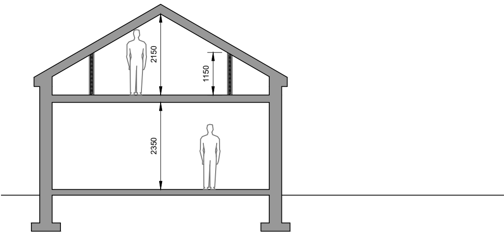
GA Cross Section
