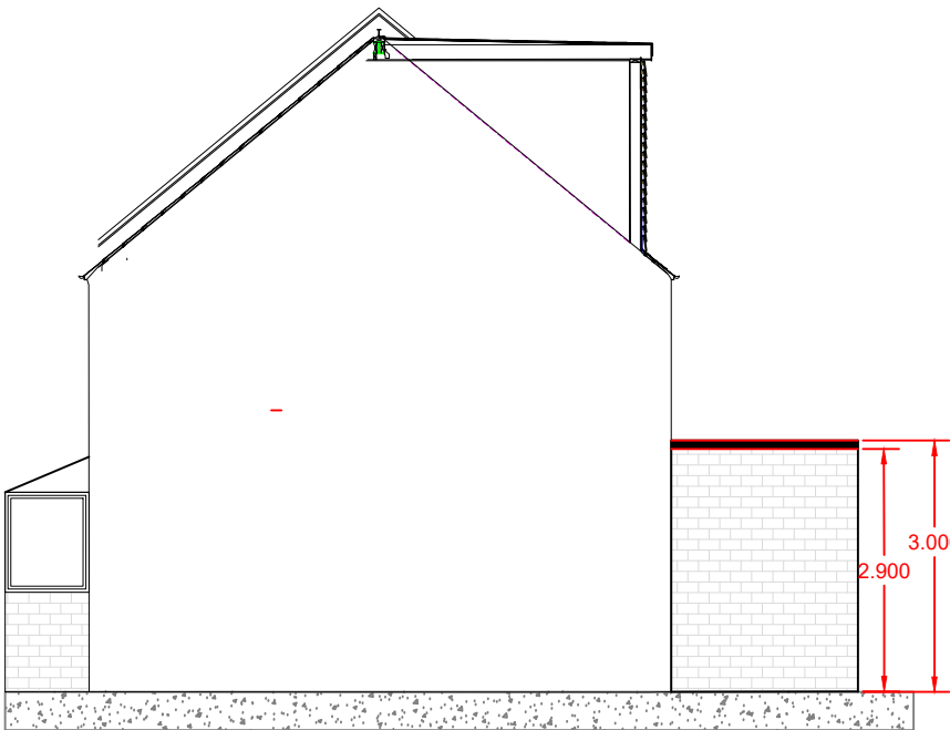
Proposed Site B Elevation with Added Space (Highlighted in Light Brickwork)
