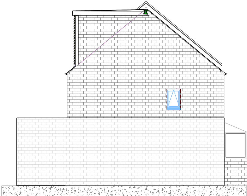
Proposed Side A Elevation Facing House No. 71 (Single Storey Rear Extension Not Visible)
