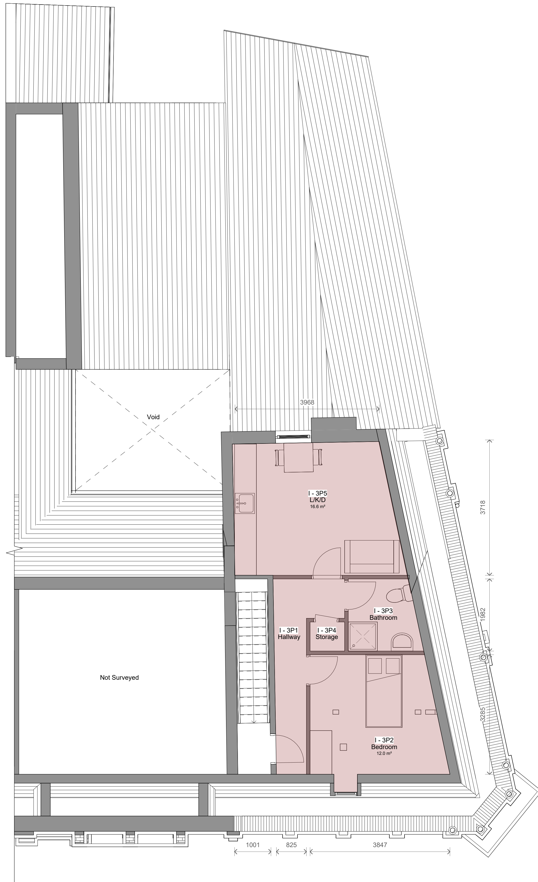
2 LEVEL 3 - Proposed 1 : 50
