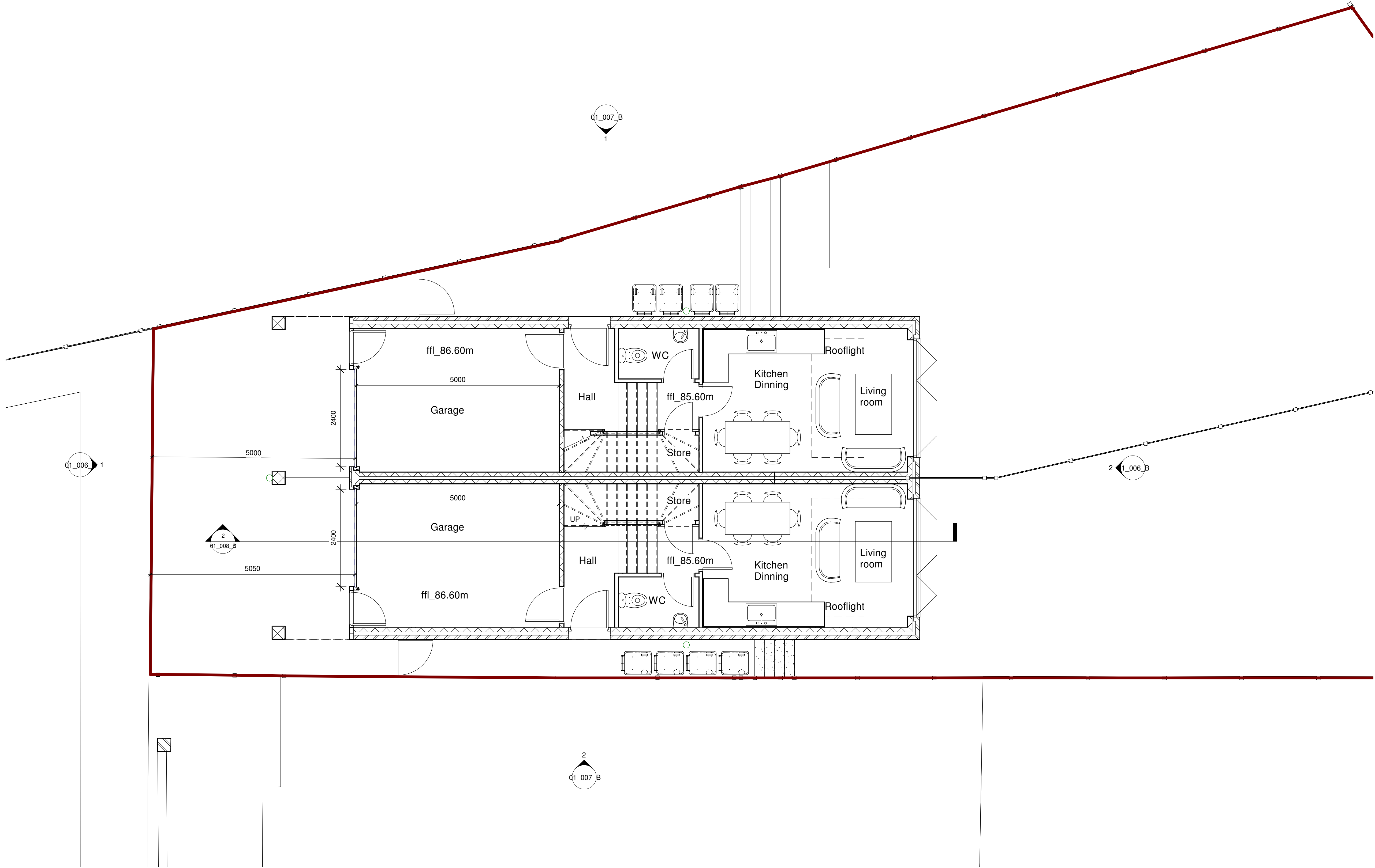
Proposed Ground Floor 1 : 50
