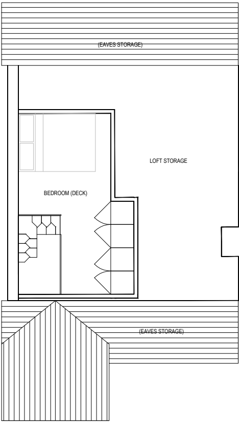
PROPOSED SECOND FLOOR PLAN (ROOF)
