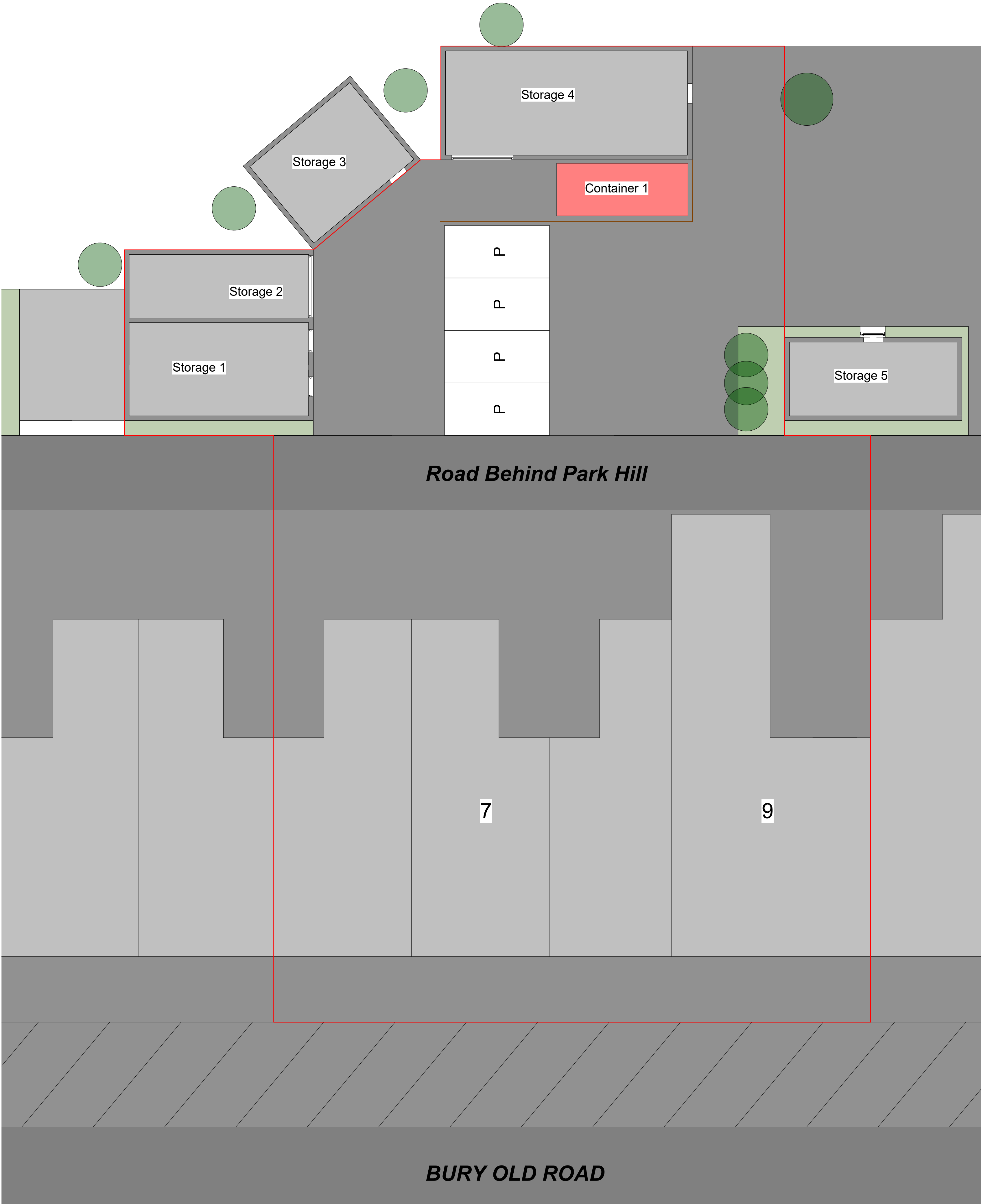
1 Level 0 - Proposed 1 : 100
