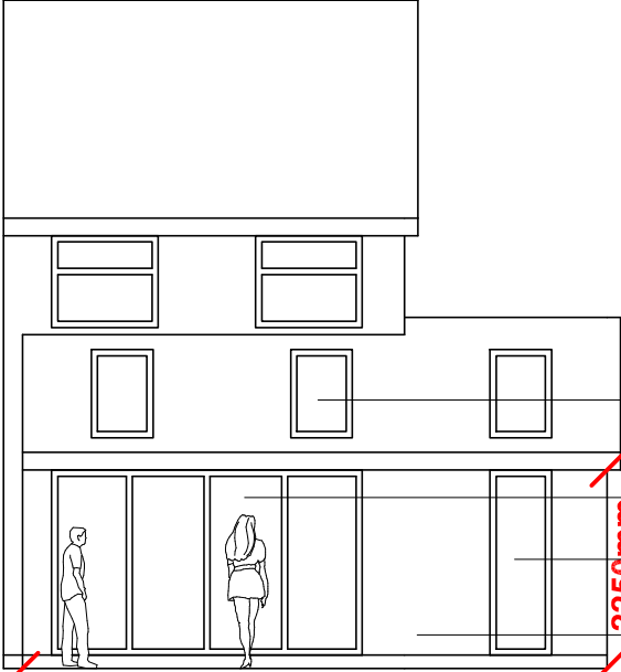
PROPOSED REAR ELEVATION 1:100
