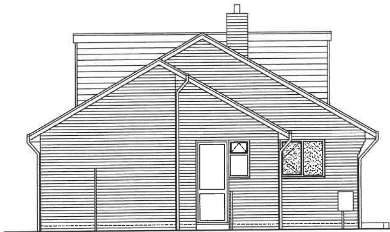
EXISTING NORTH WEST ELEVATION 1:100 @ A4
