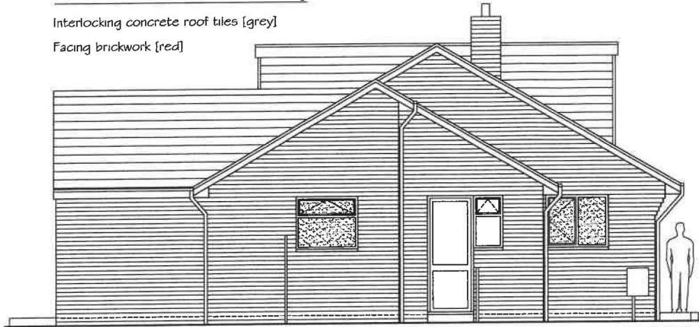
PROPOSED NORTH WEST ELEVATION 1:100 @ A4
