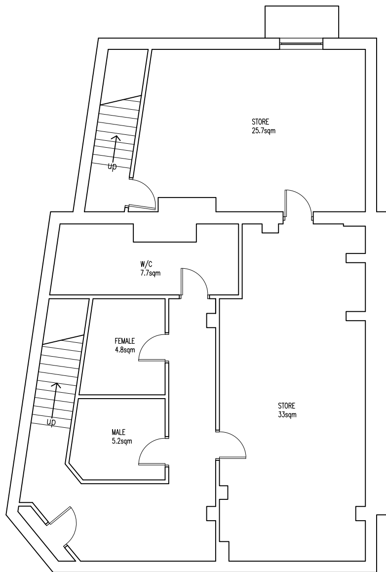
EXISTING BASEMENT FLOOR PLAN 1:100 @ A3
