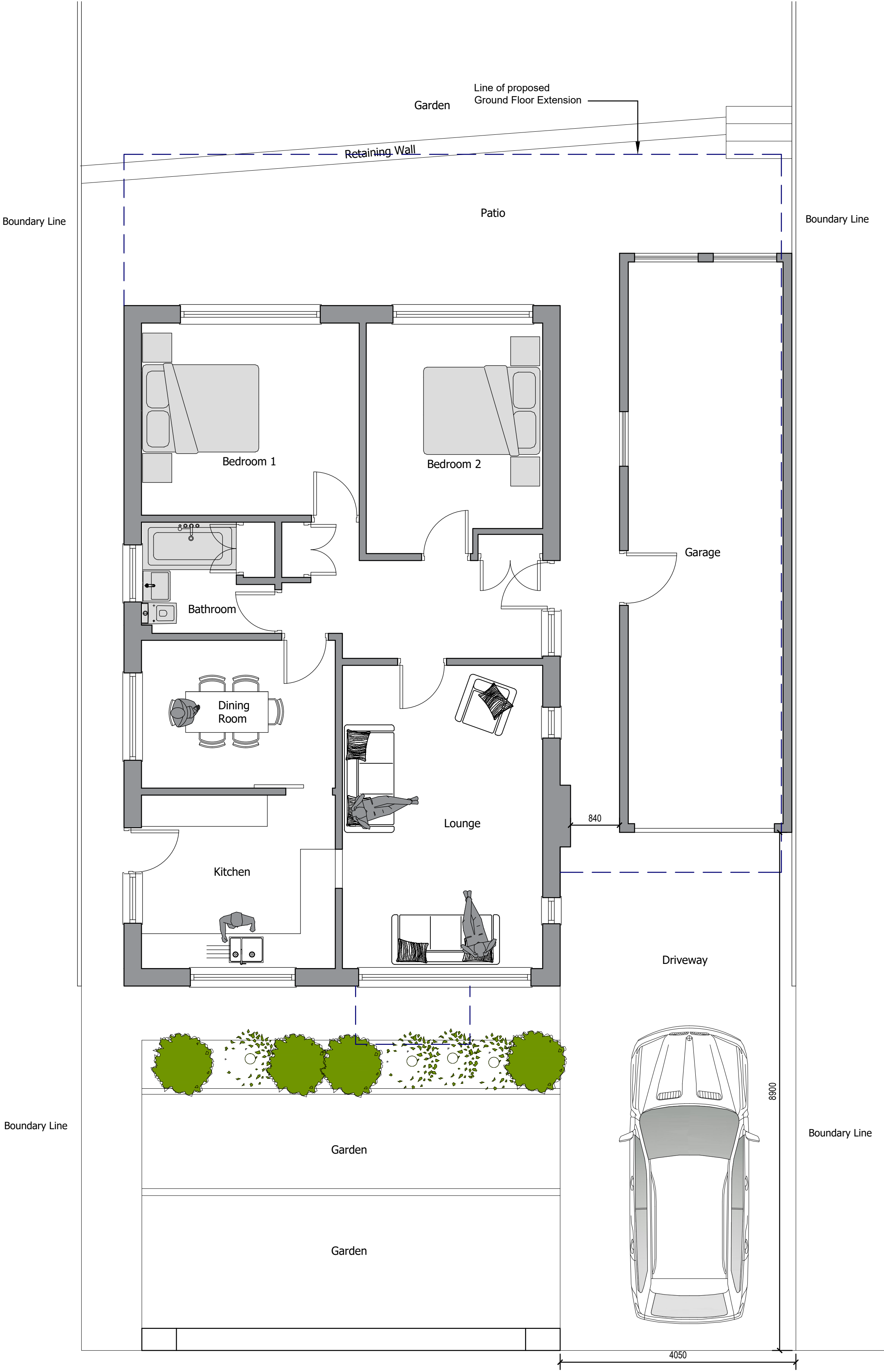
Ground Floor
