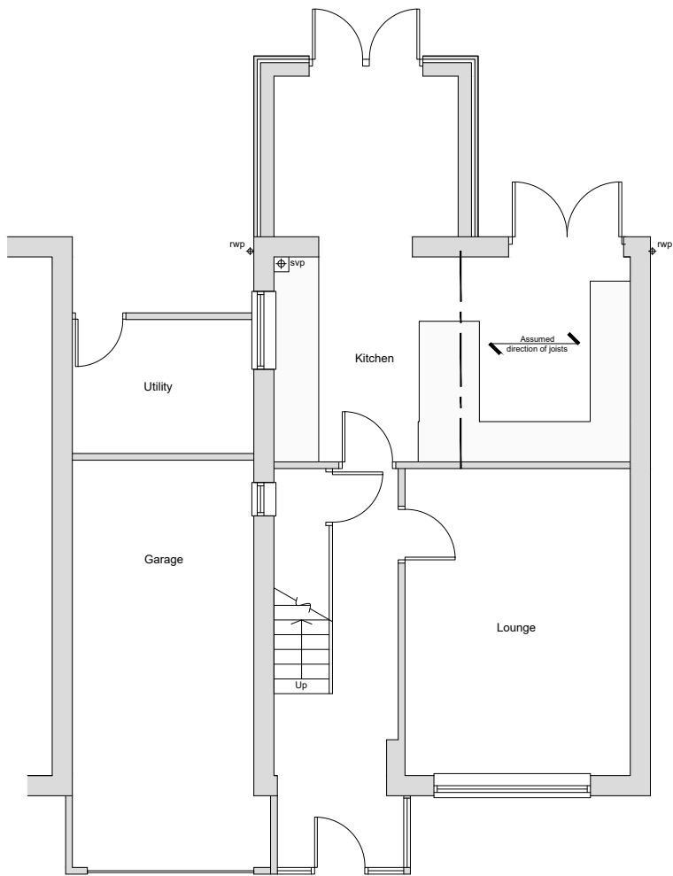
Existing GF Plan 0m 1 2 3 4 5m
